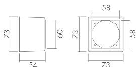
Abmessungen in mm
